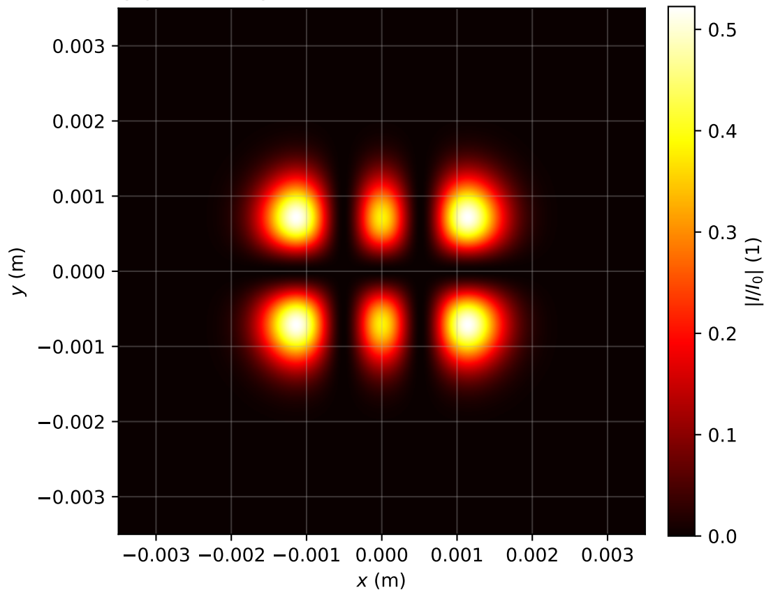
Intensity profile I(x, y, z = 2.070)/I_0 , P_{in}=0.5P_{cr} , artificial time
